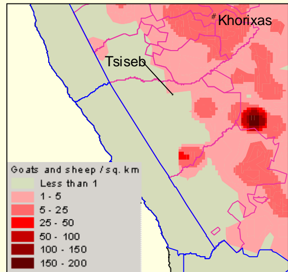
Non-wildlife population densities in and around Tsiseb conservancy. State protected areas are outlined in blue, conservancies in purple.
