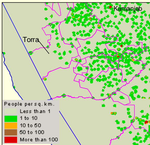
Non-wildlife population densities in and around Torra conservancy. State protected areas are outlined in blue, conservancies in purple.
